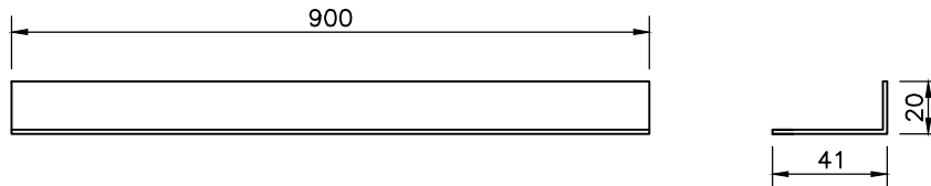
BOTTOM CROWN SUPPORT QTY:-2NOS.
