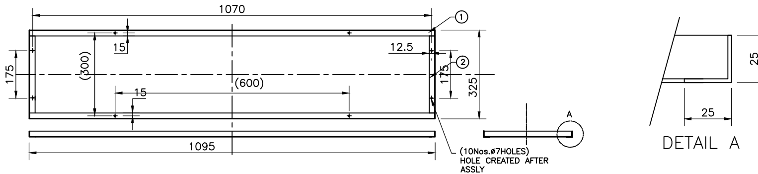
MIDDLE BOTTOM FRAME
